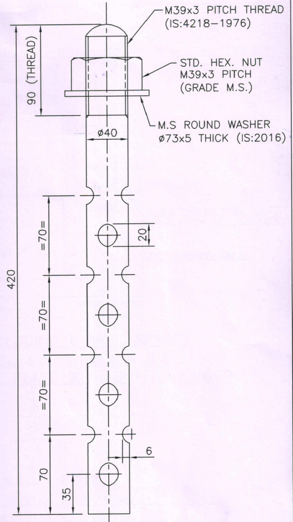
ANCHOR BOLT 150 NOS. REQUIRED THUS (INCLUDING 6 NOS. SPARE) MATERIAL- MILD STEEL
