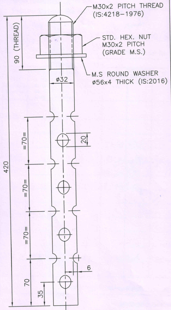
ANCHOR BOLT 212 NOS. REQUIRED THUS (INCLUDING 10 NOS. SPARE) MATERIAL- MILD STEEL
