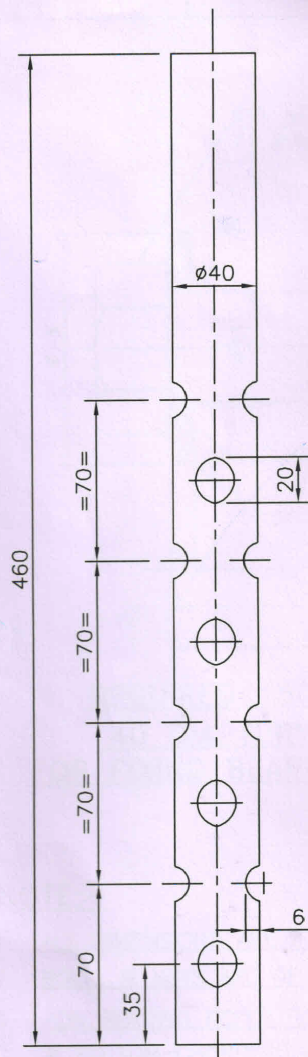
ANCHOR PIN 80 NOS. REQUIRED THUS (INCLUDING 8 NOS. SPARE) MATERIAL- MILD STEEL
