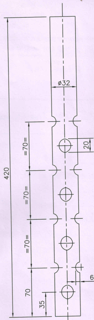
ANCHOR PIN 106 NOS. REQUIRED THUS (INCLUDING 10 NOS. SPARE) MATERIAL- MILD STEEL
