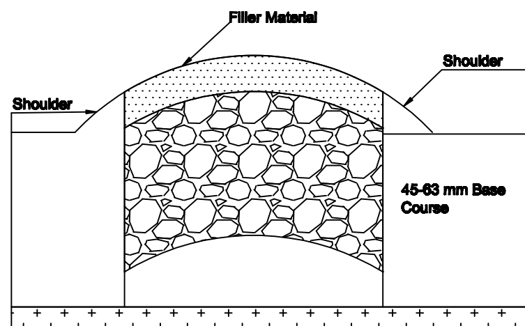
Cross section of Road
