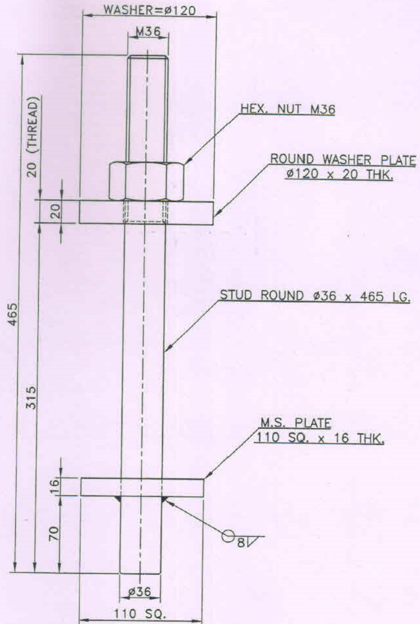
DETAILS OF H.D. BOLTS 1560 NOS. REQD. INCLUDING 24 NOS. SPARE
