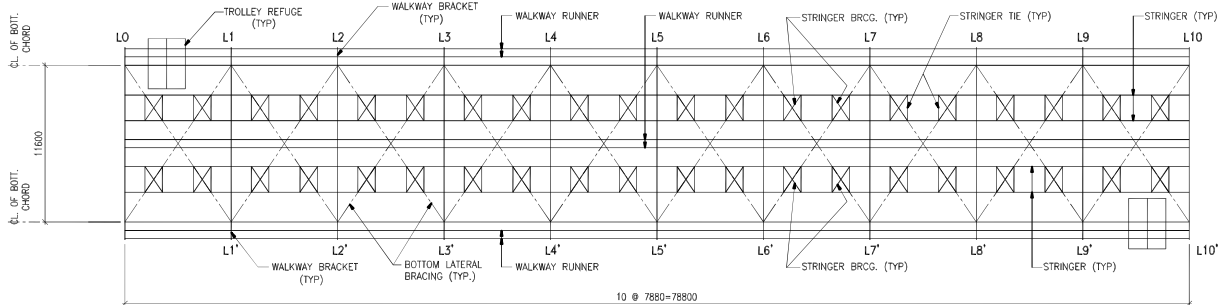
PLAN AT STRINGER LEVEL
