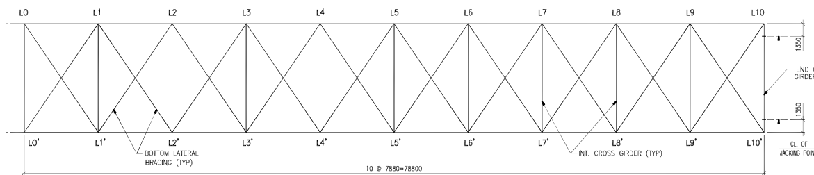
PLAN AT BOTTOM CHORD LEVEL
