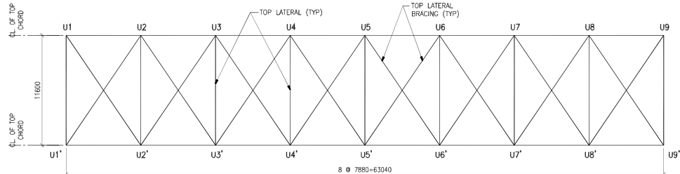
TOP PLAN
